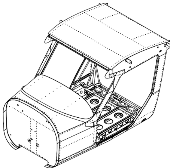
Figure 3.6.2.2. Cockpit Structure.
